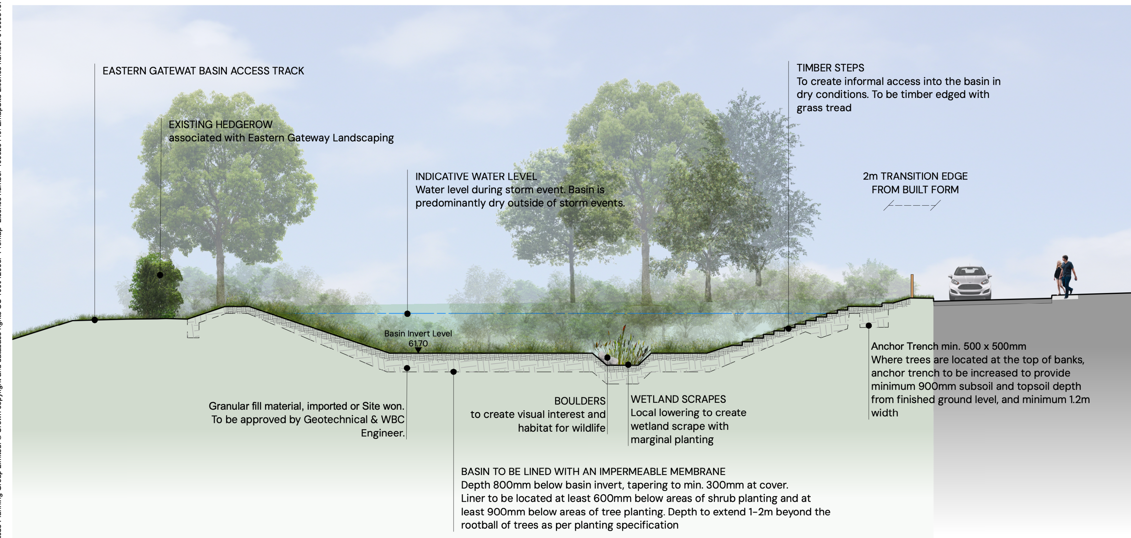
SECTION B-BB
