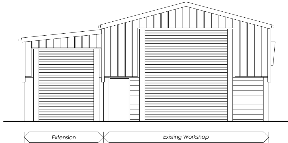
Front Elevation - Northwest
