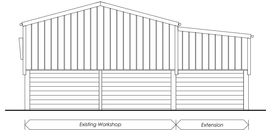
Rear Elevation - Southeast
