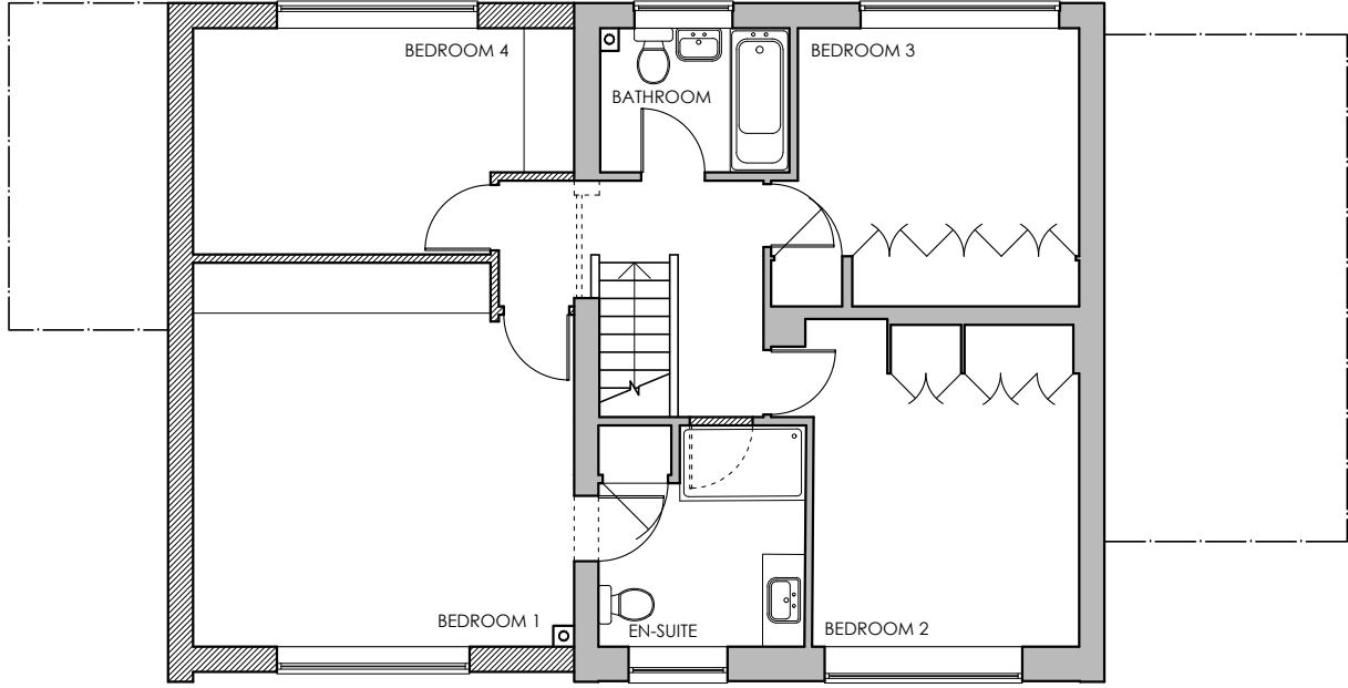
FIRST FLOOR PLAN 1:100
