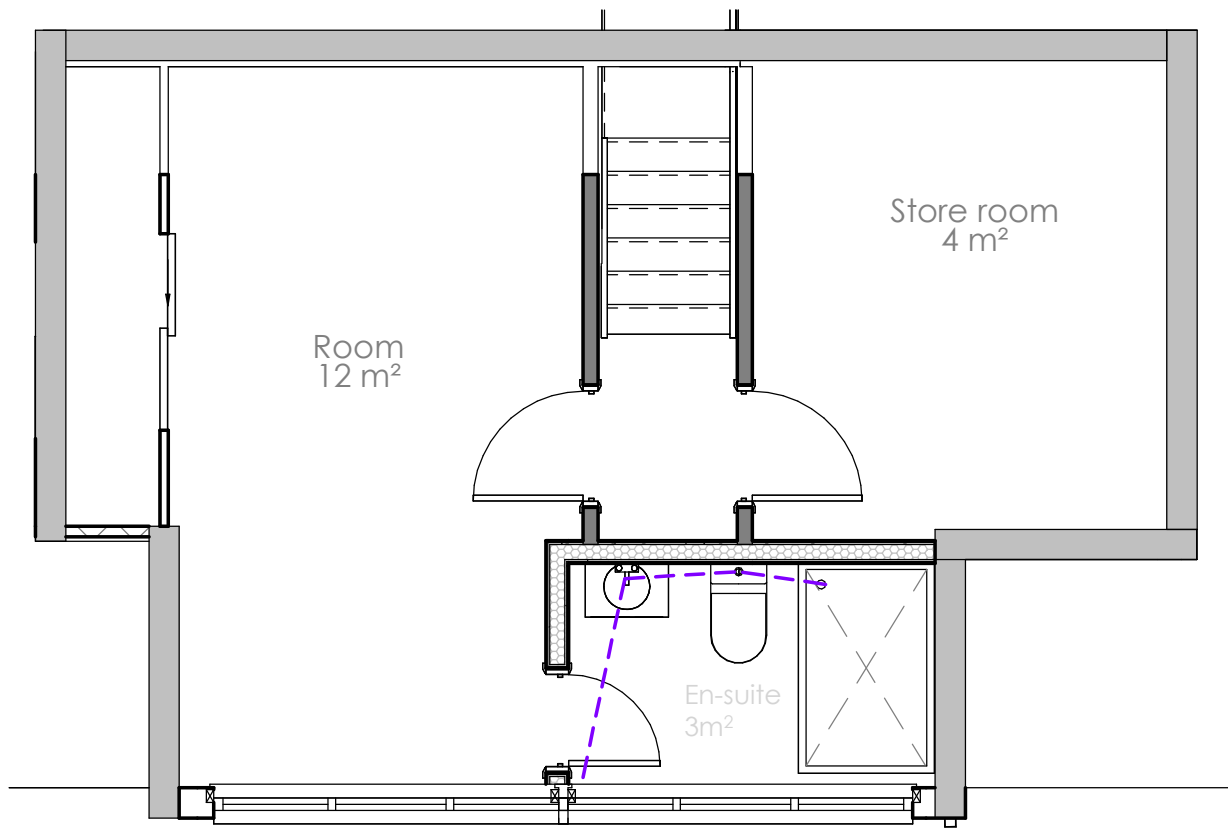
Level 2 - Proposed 1 : 50
