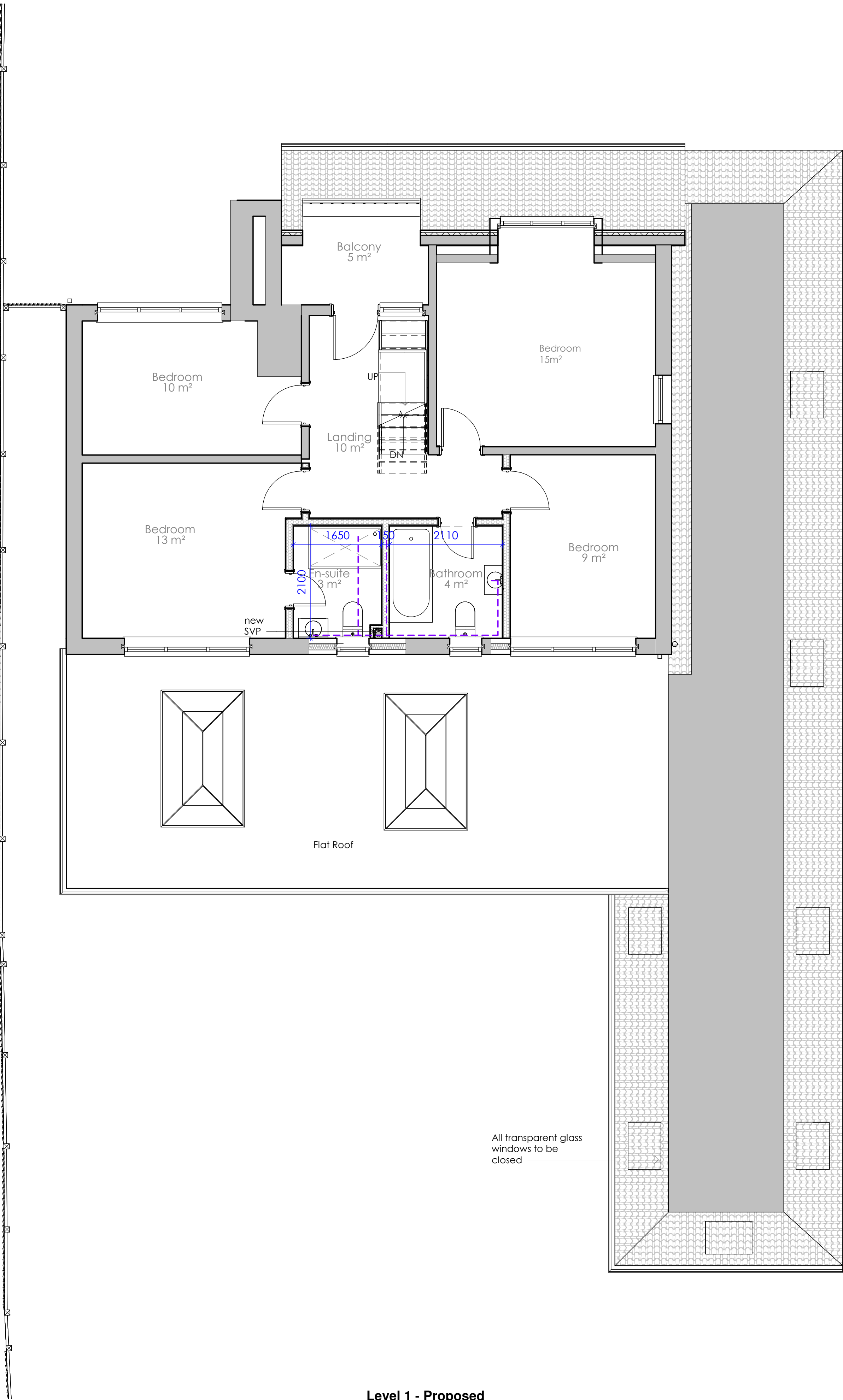
Level 1 - Proposed 1 : 50
