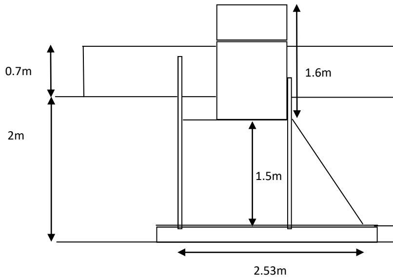
Side View — Proposed Construction
