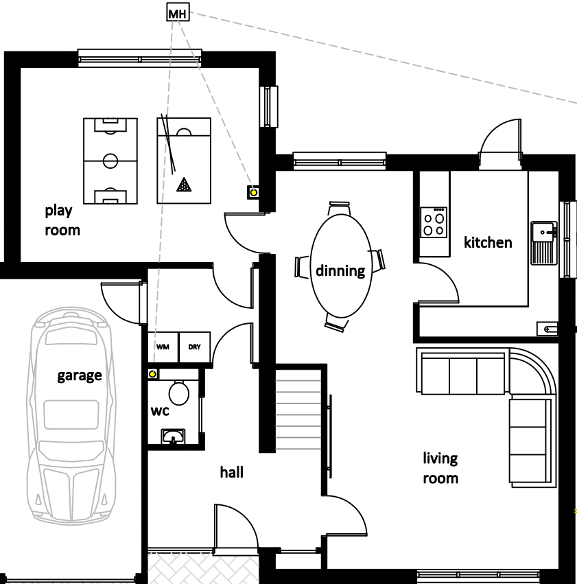
Ground 1:100
