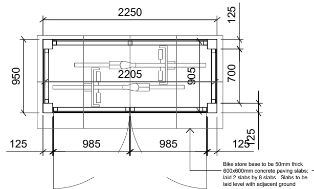
CYCLE STORE - Plan (1:50)
