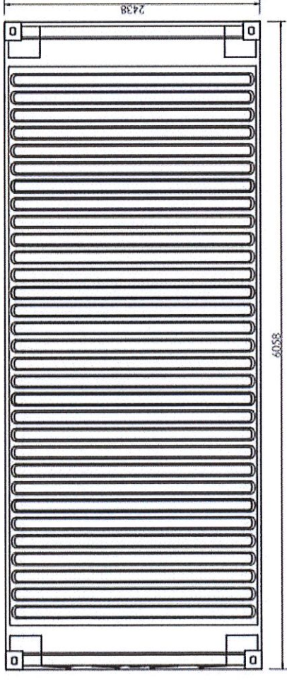
20ft Shipping Container - Roof Plan
