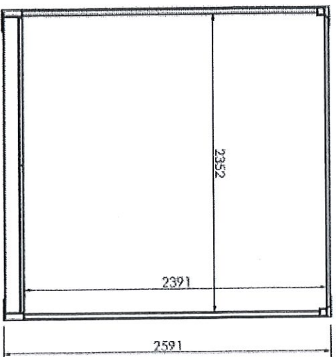
20ft Shipping Container - Section
