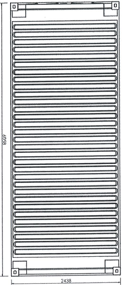
20ft Shipping Container - Roof Plan
