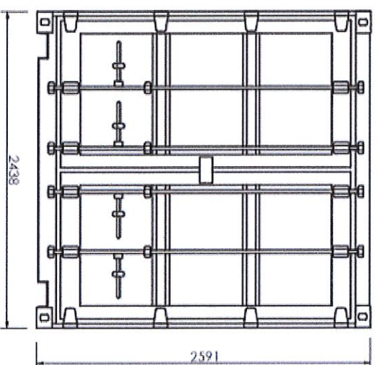
20ft Shipping Container - Door Elevation
