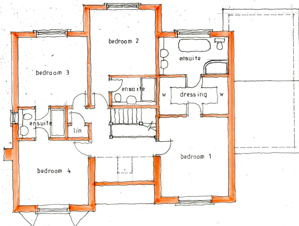
FIRST FLOOR
