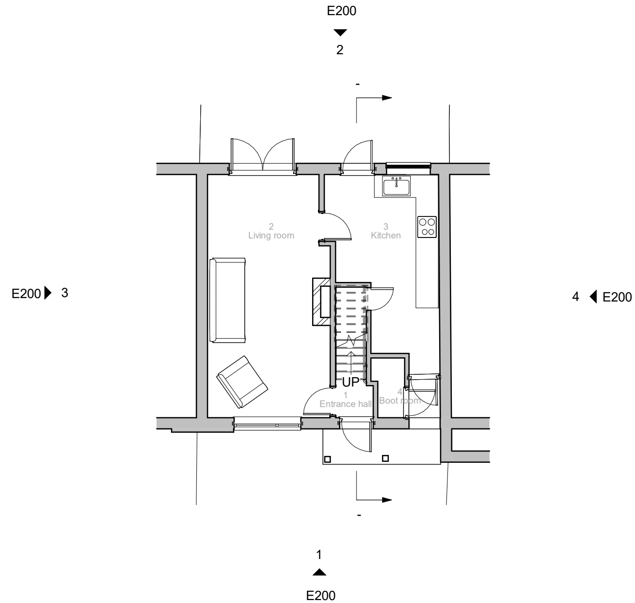
1 Ground 1 : 100
