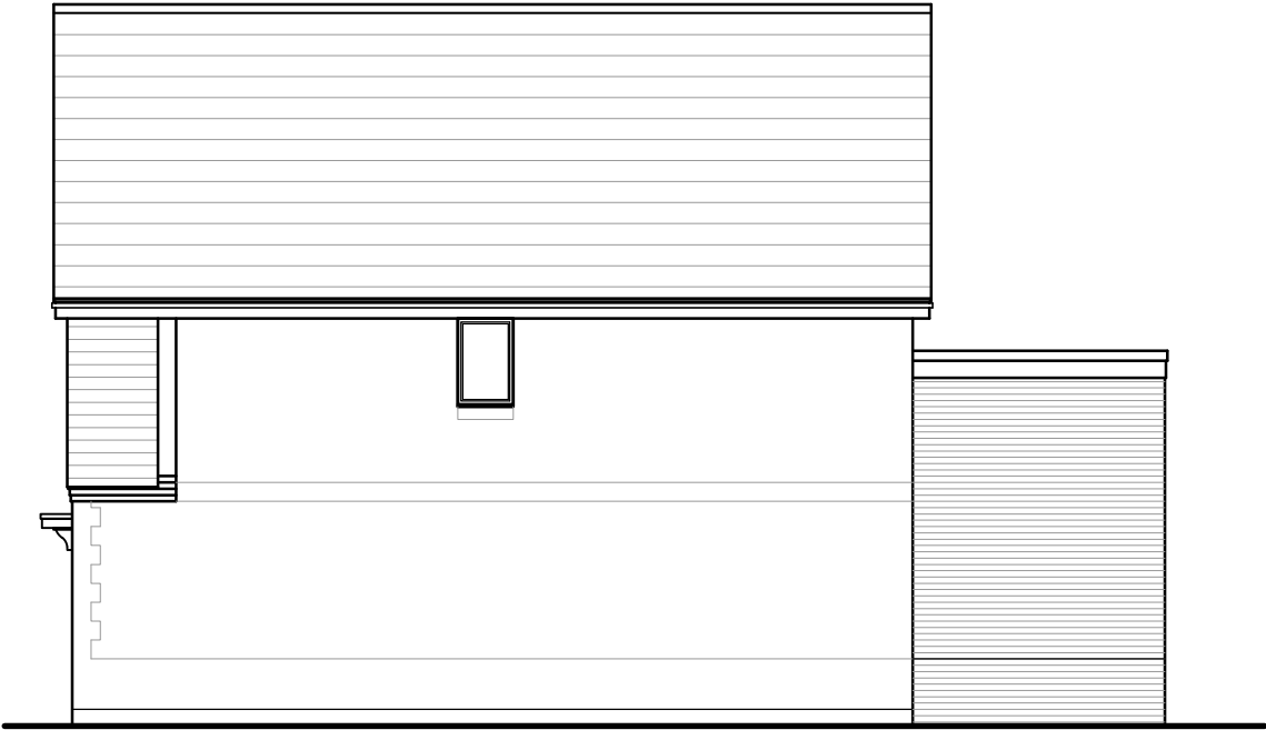
EAST ELEVATION
