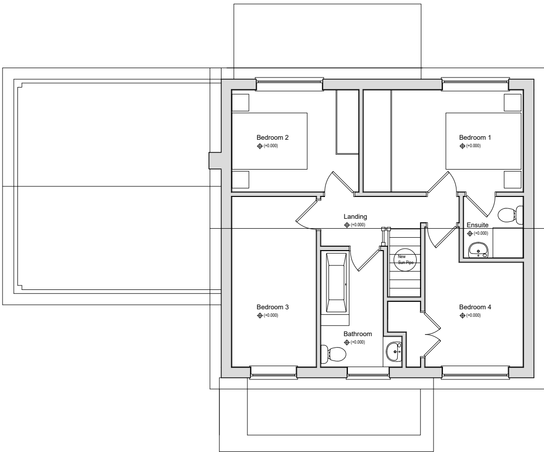
02 Existing First Floor Plan 1:100
