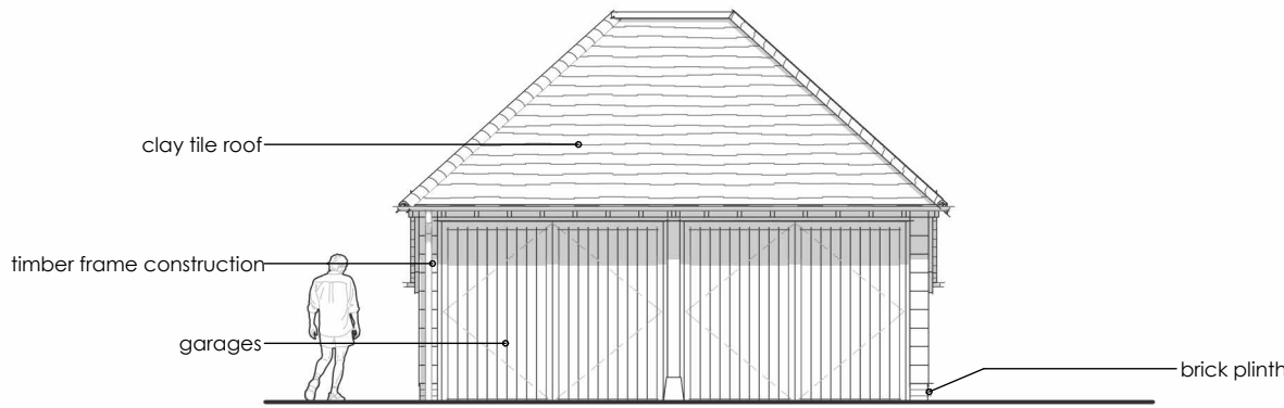
North-East Elevation
