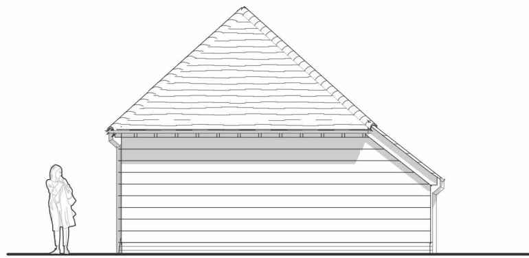
North-West Elevation
