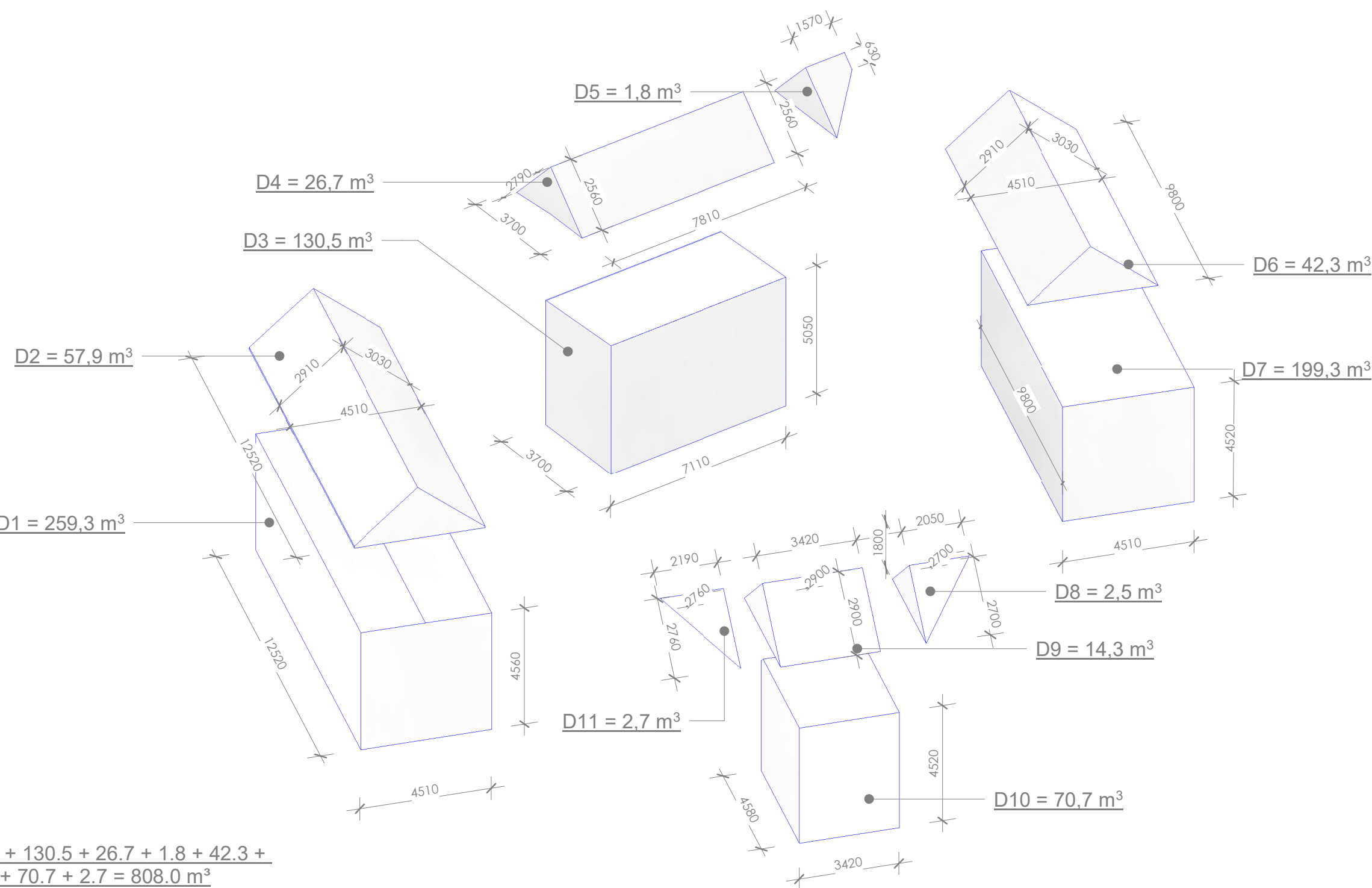
OVERALL PROPOSED VIEW 1
