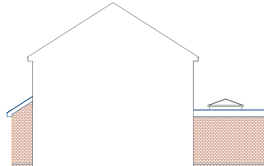
Proposed Side Elevation (R)
