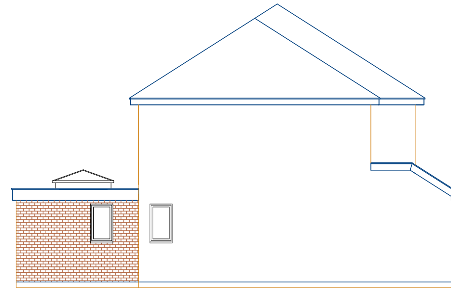
Proposed Side Elevation (L)
