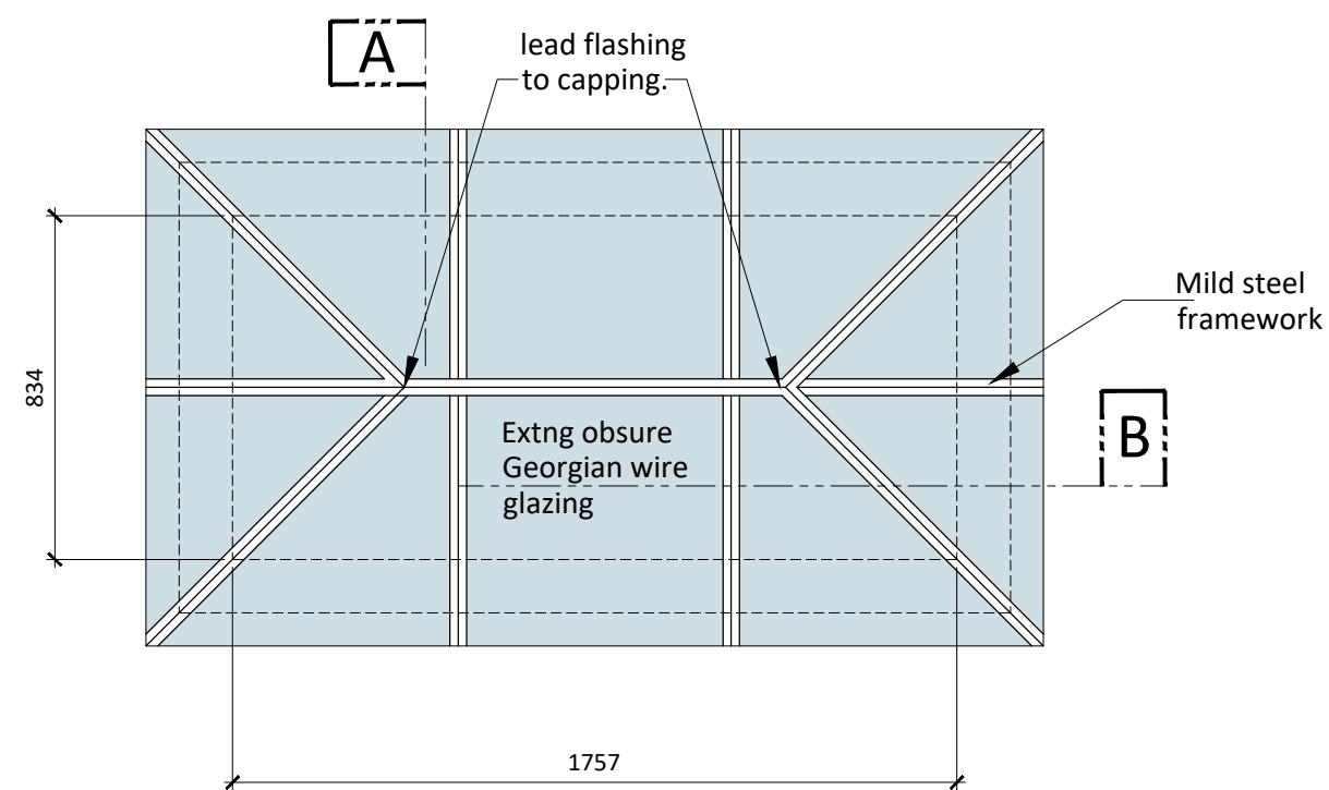
Typical Roof Lantern
