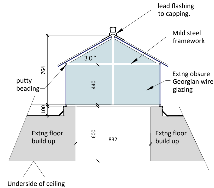
Typical Section A
