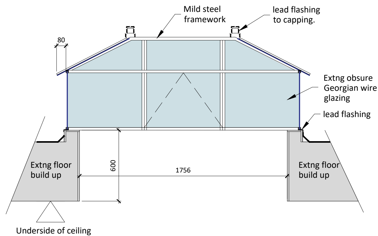
Typical Section B
