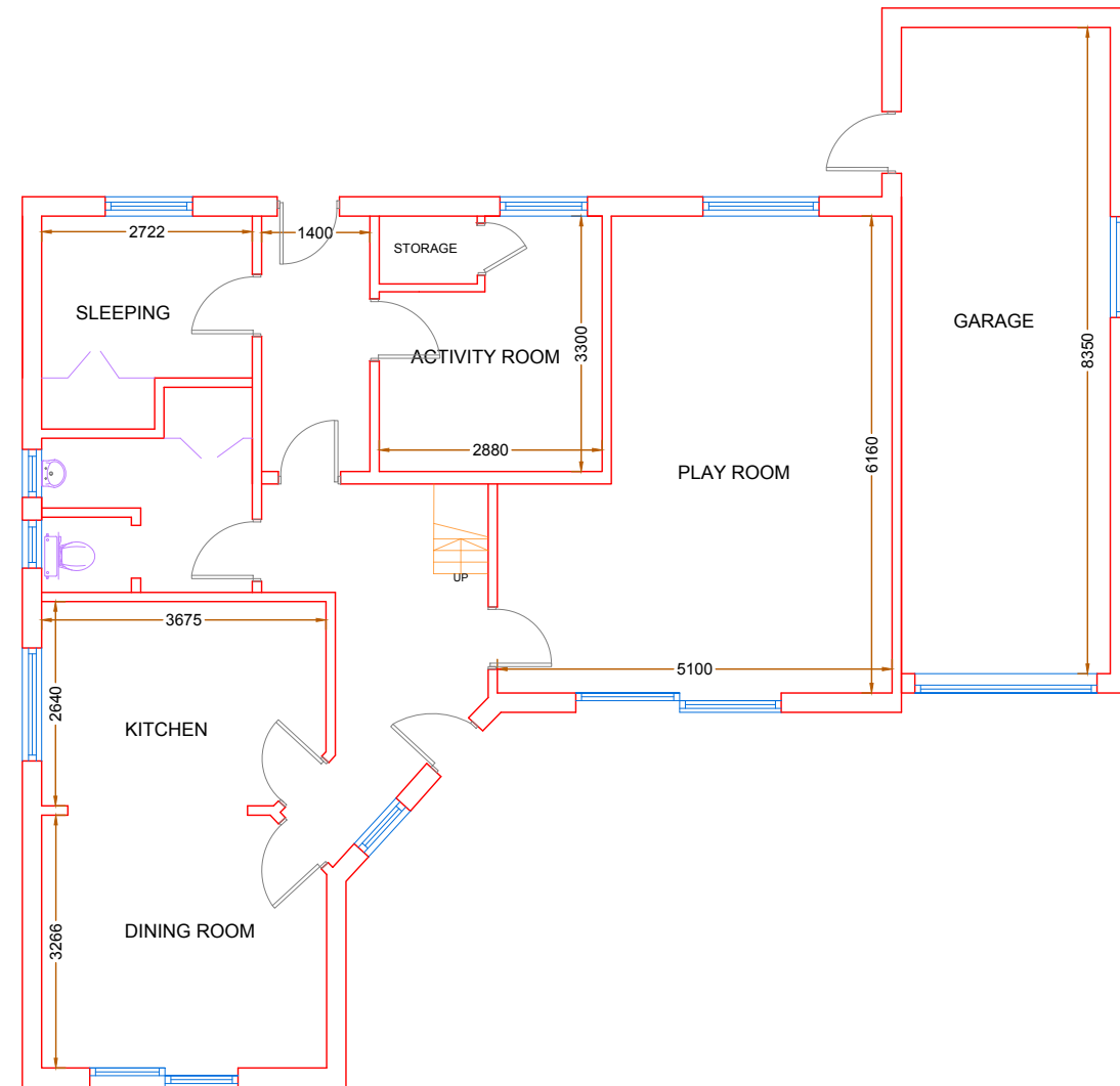
FLOOR PLAN AS PROPOSED
