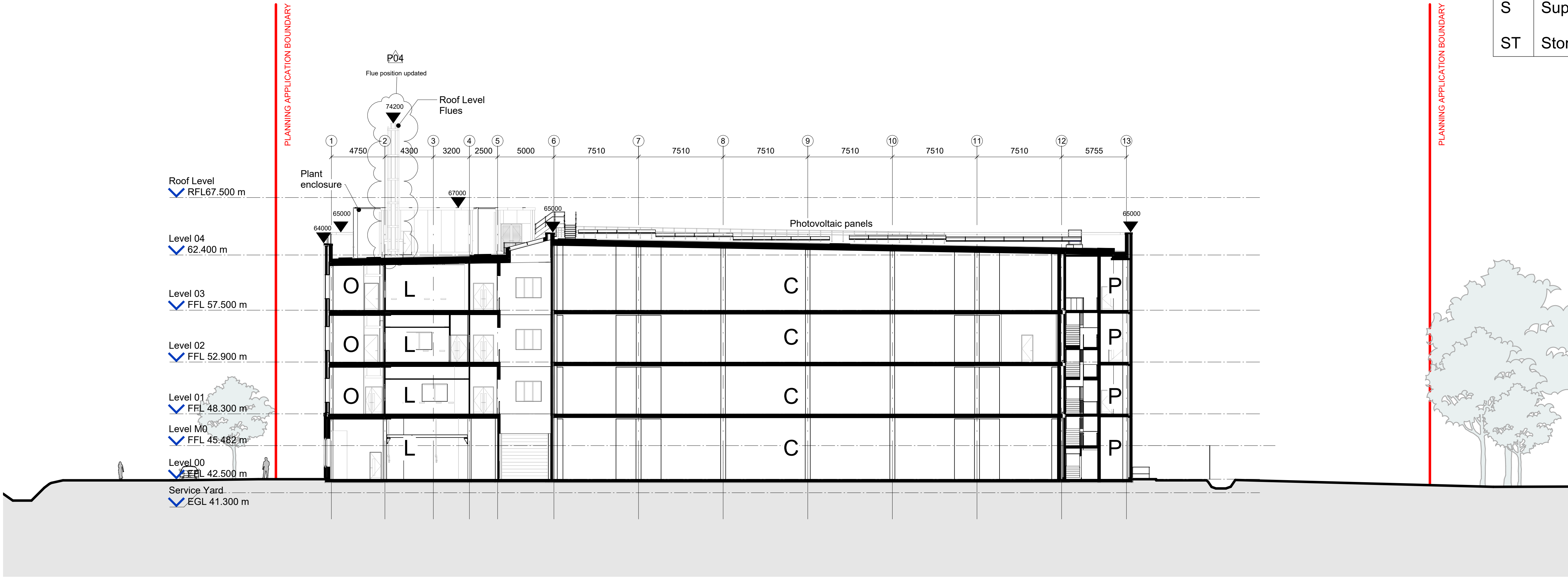
1 Section AA 1 : 200 0 4 8 m Scale 1:200
