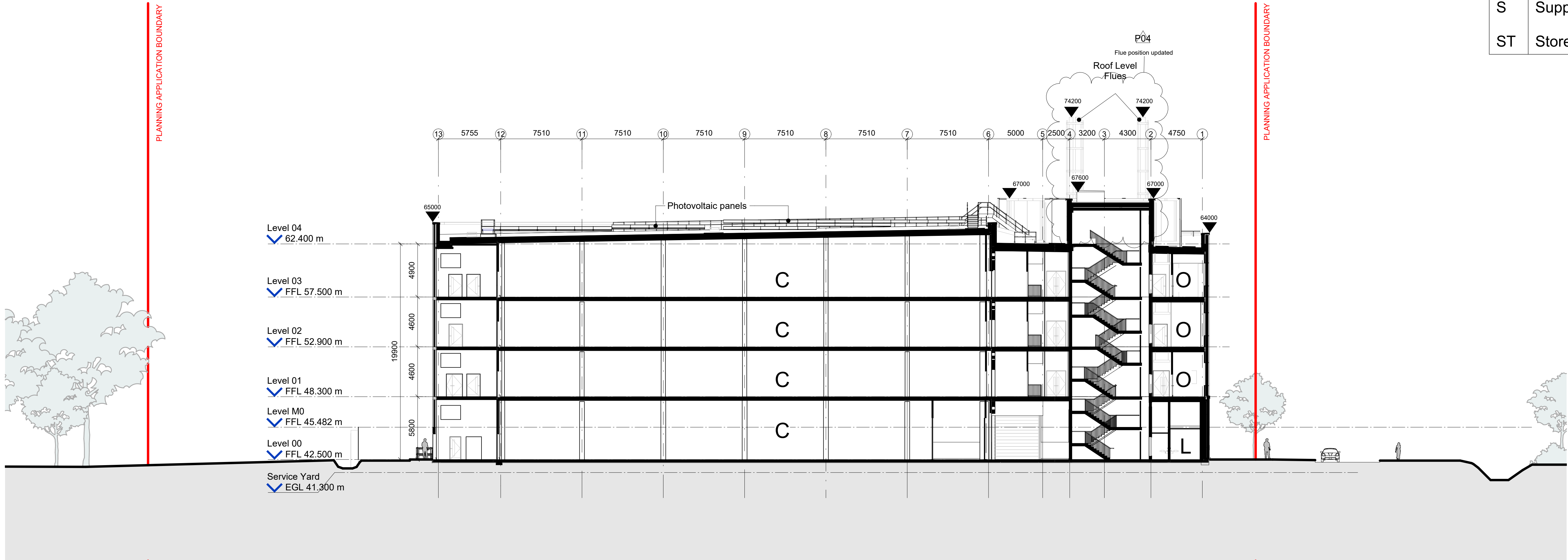
1 Section F-F 1 : 200 0 4 8 m Scale 1:200
