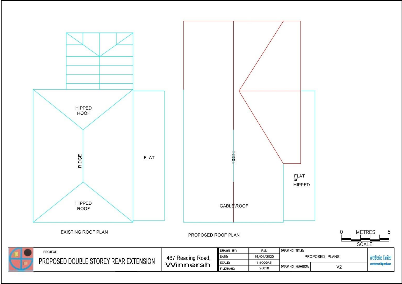
Figure 2 – Existing and proposed roof plans
