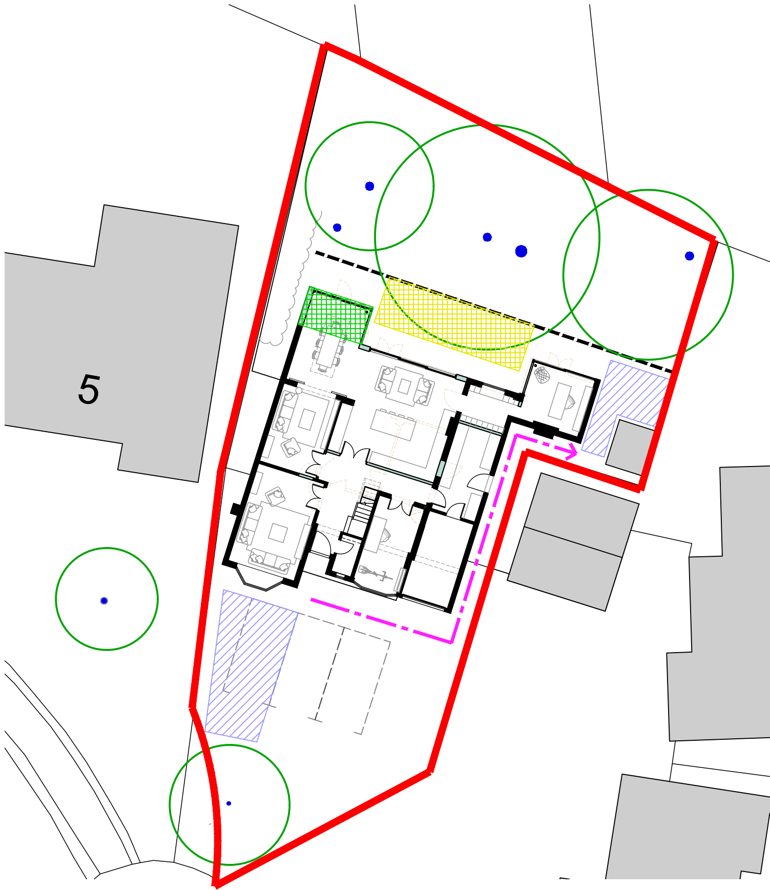
TREE PROTECTION PLAN @ 1200
