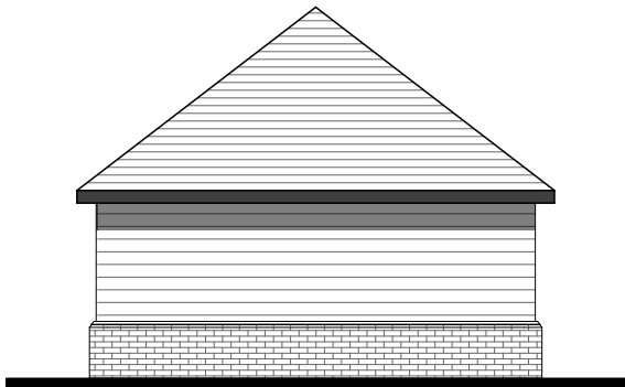
SIDE ELEVATION 1:100 Brooklands, Warren Lane, Finchampstead RG40 4HS
