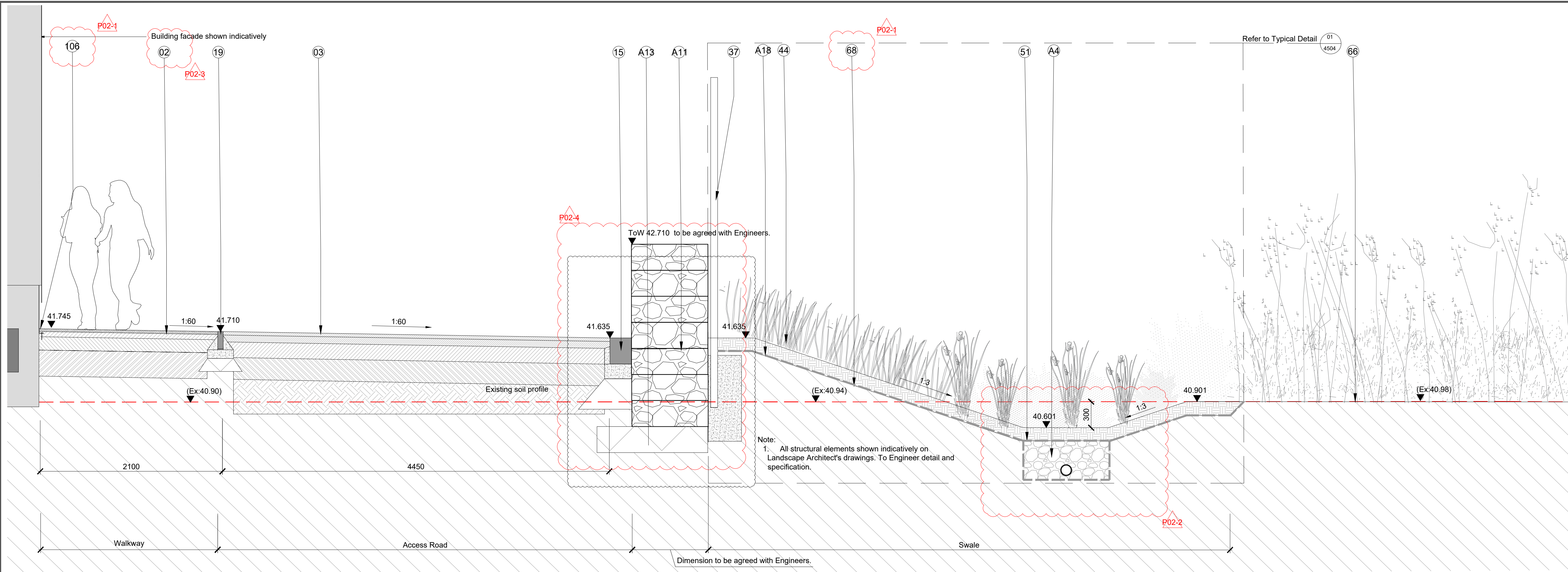
01 Section 5 - Service road and swale scale 1:25 @ A1
