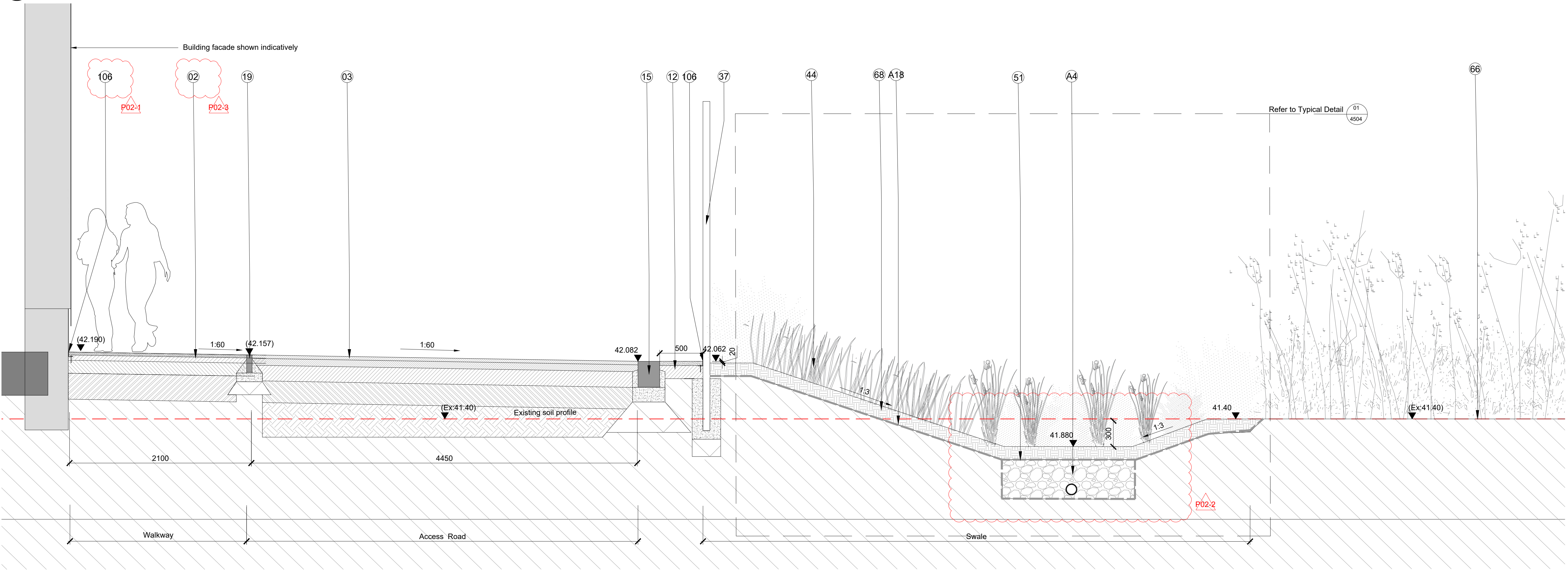
02 Section 4 - Service road and swale scale 1:25 @ A1
