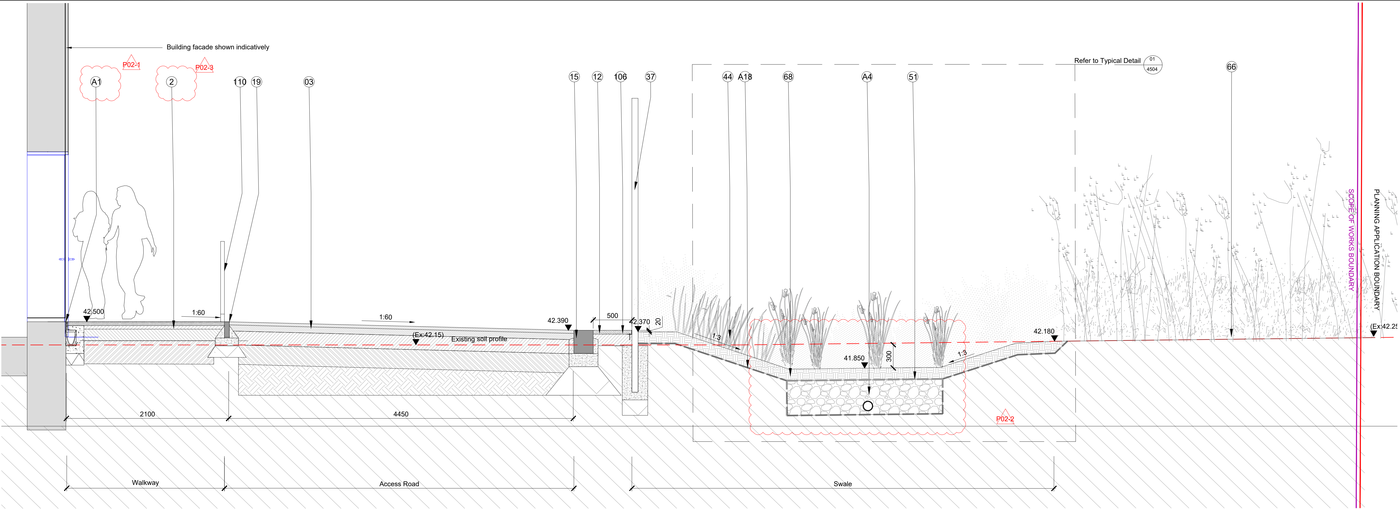
01 Section 3 - Service road and swale scale 1:25 @ A1
