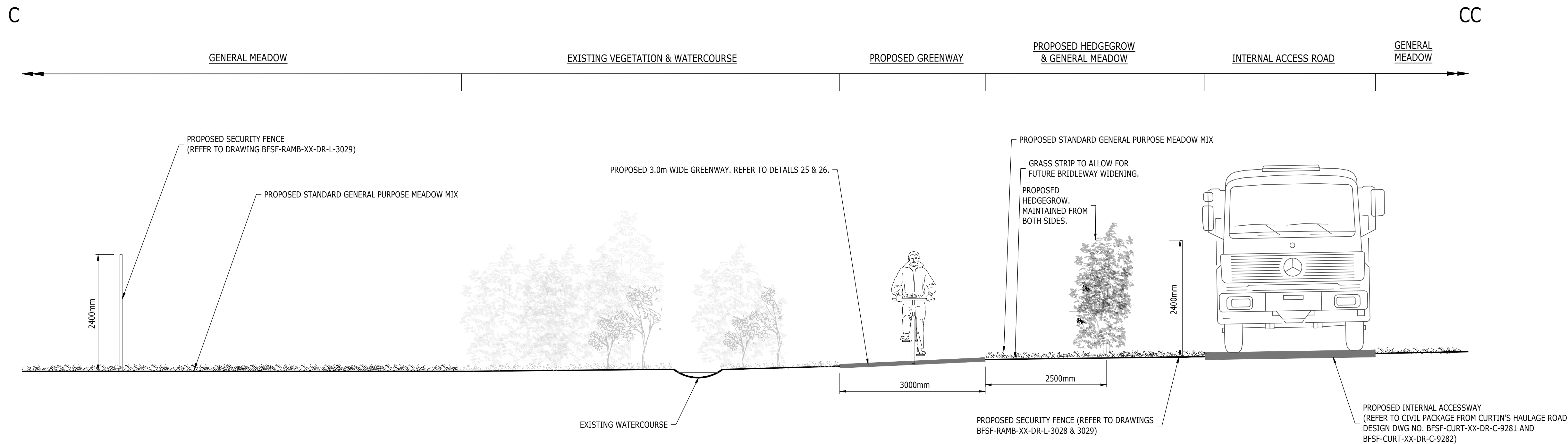
03 PROPOSED GREENWAY & INTERNAL SITE ACCESSWAY SECTION NOT TO SCALE
