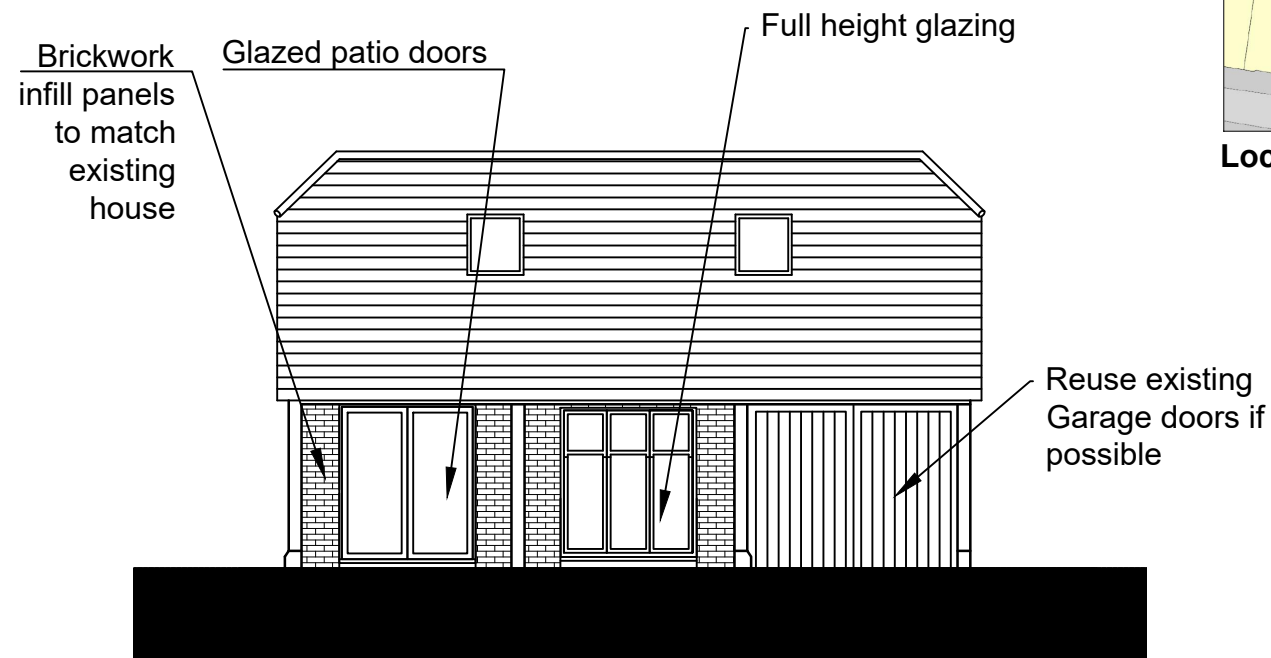
South elevation
