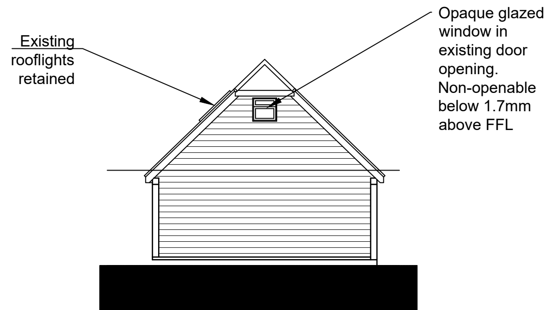
East elevation
