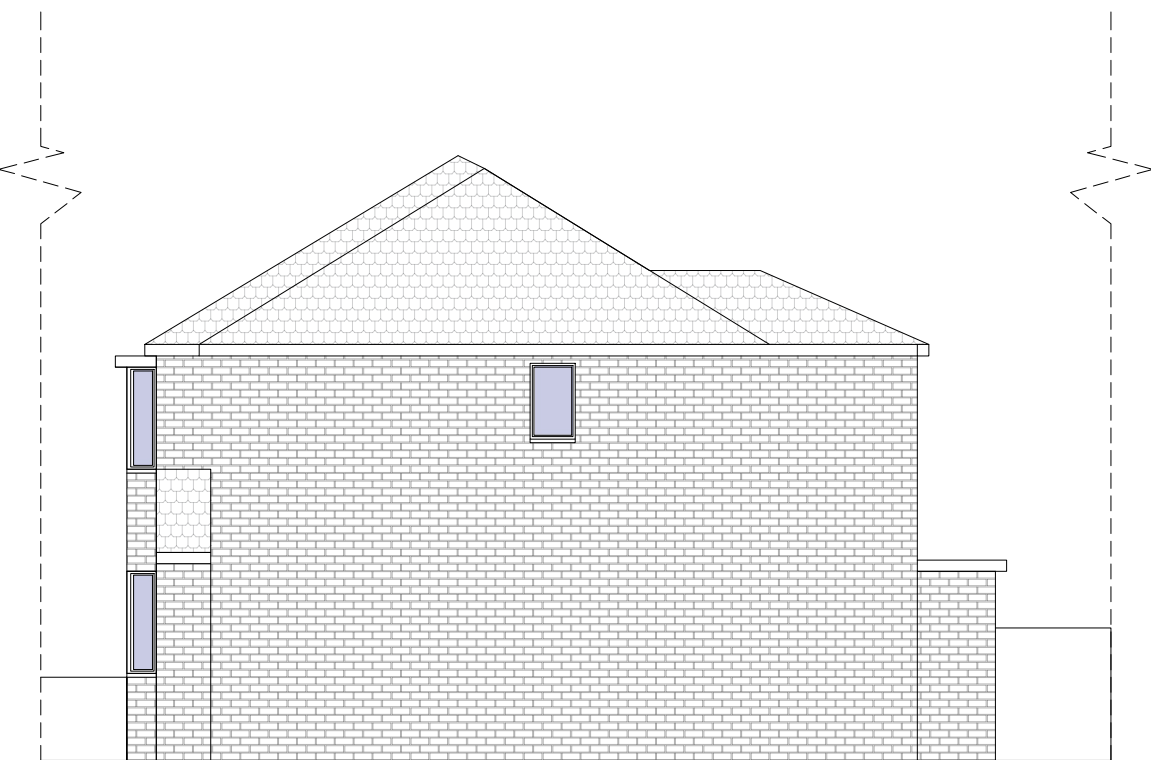
Proposed West Elevation (No Proposed Change)
