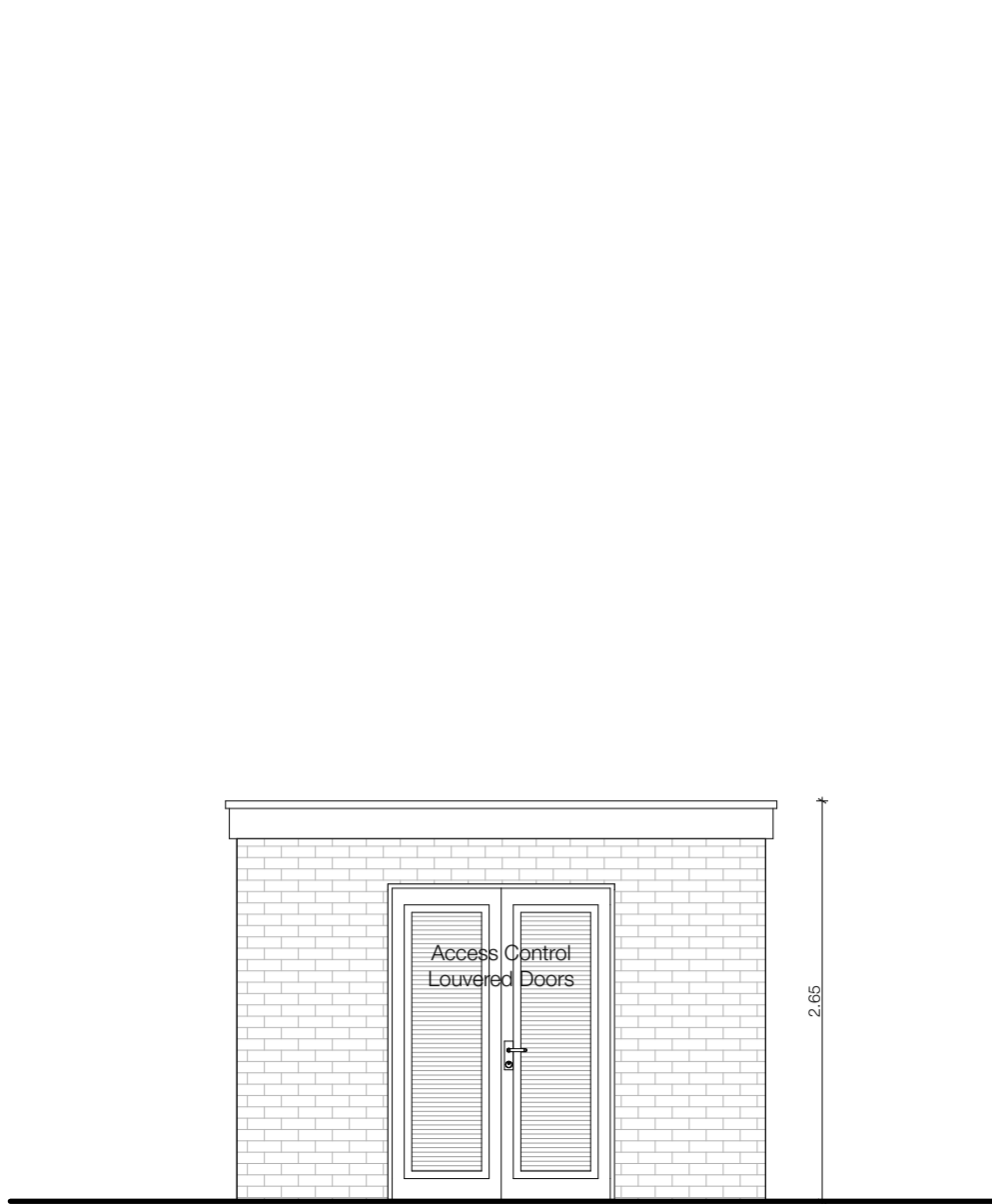
Front (South East) Elevation
