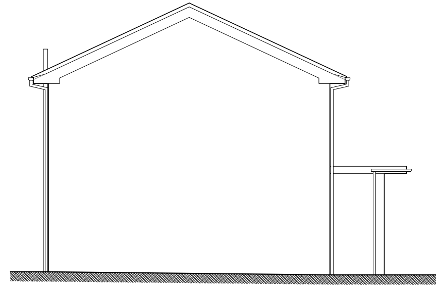
Existing South East (Side) Elevation
