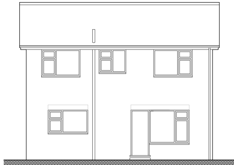
Existing South West (Rear) Elevation
