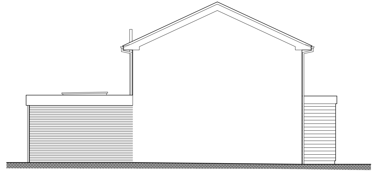
Proposed South East (Side) Elevation
