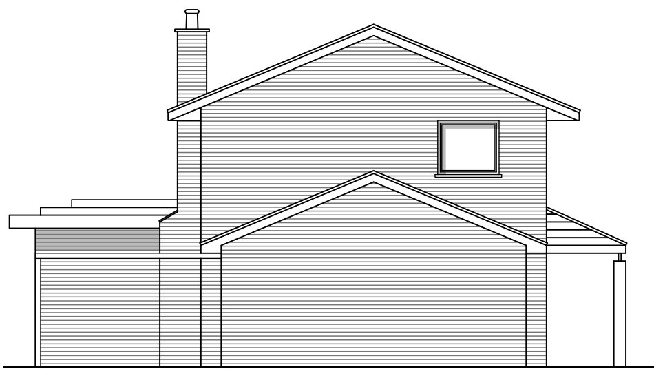
SIDE ELEVATION (NORTH-EAST FACING)
