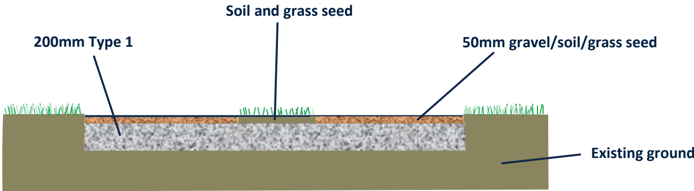
Section through driveway
