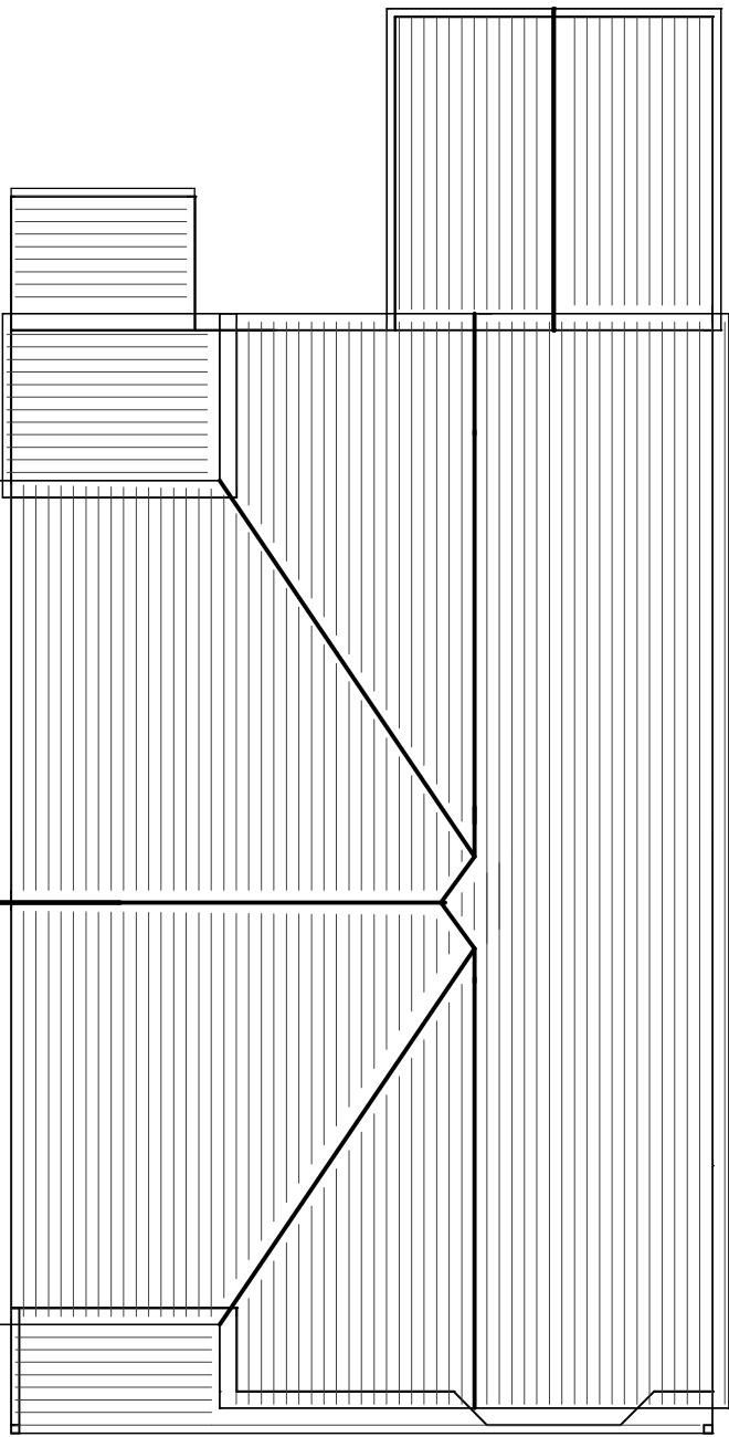
ROOF PLAN
