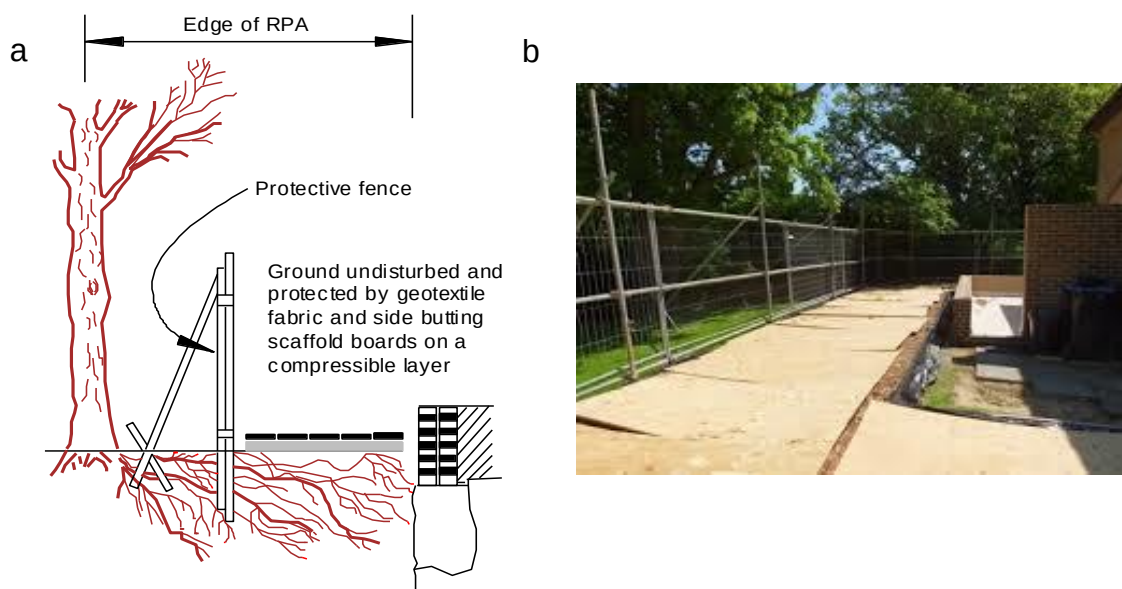
Figure 3: a. Diagrammatic illustration of ground protection within the RPA b. example of temporary ground protection.
