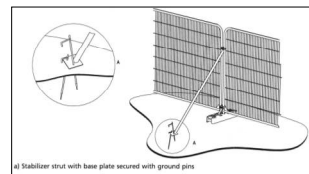
stabilizer strut with base plate secured with ground pins
