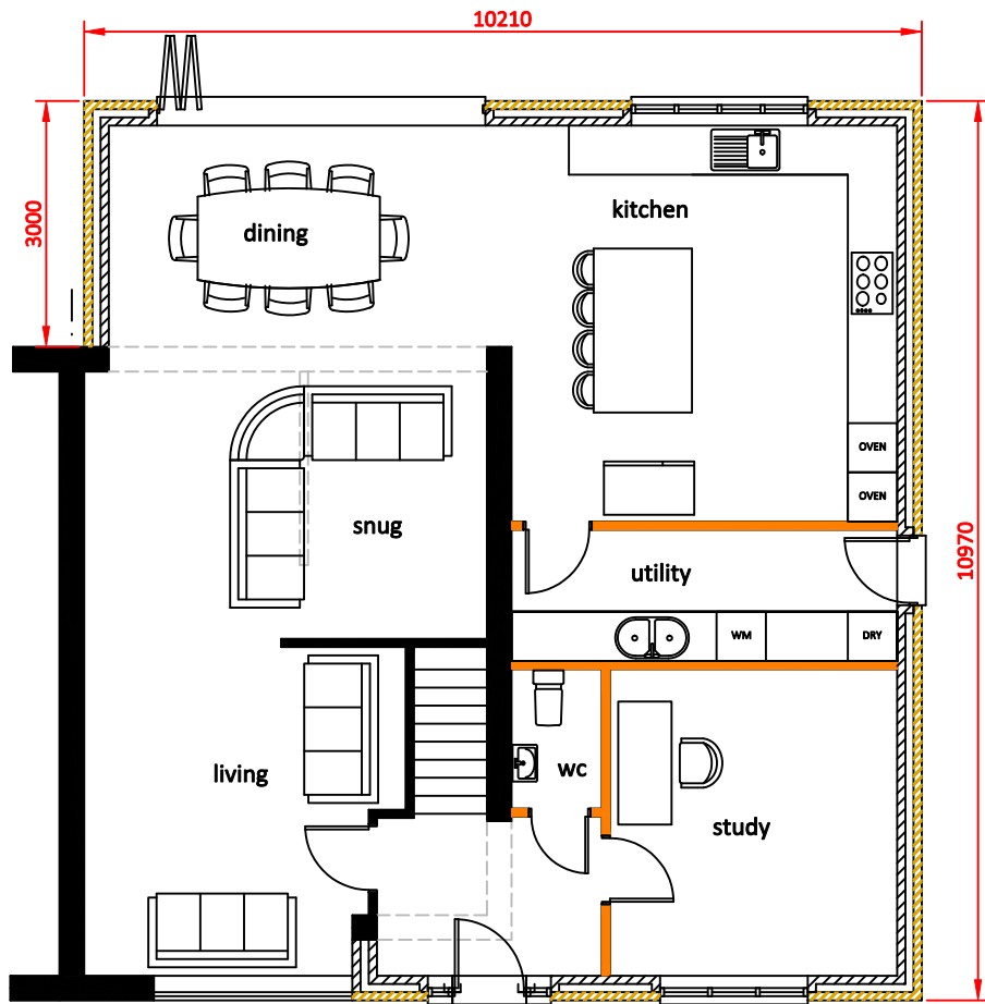
Ground 1:100
