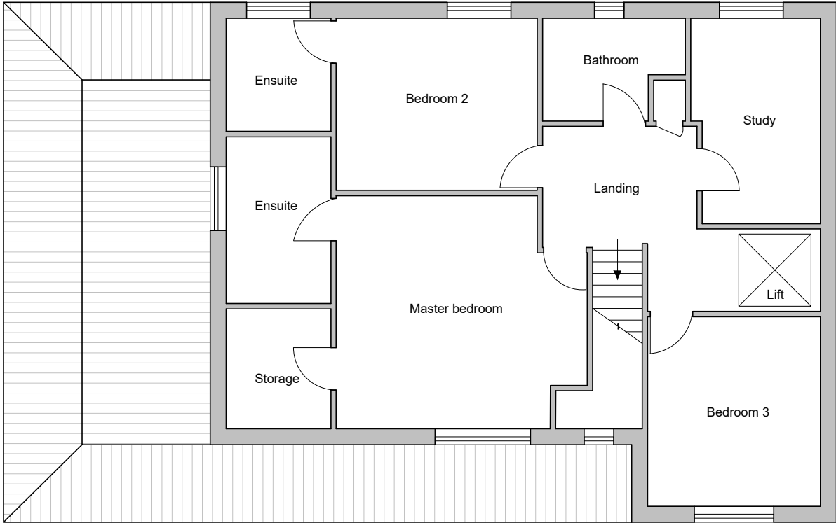
'As EXISTING' FIRST FLOOR PLAN
