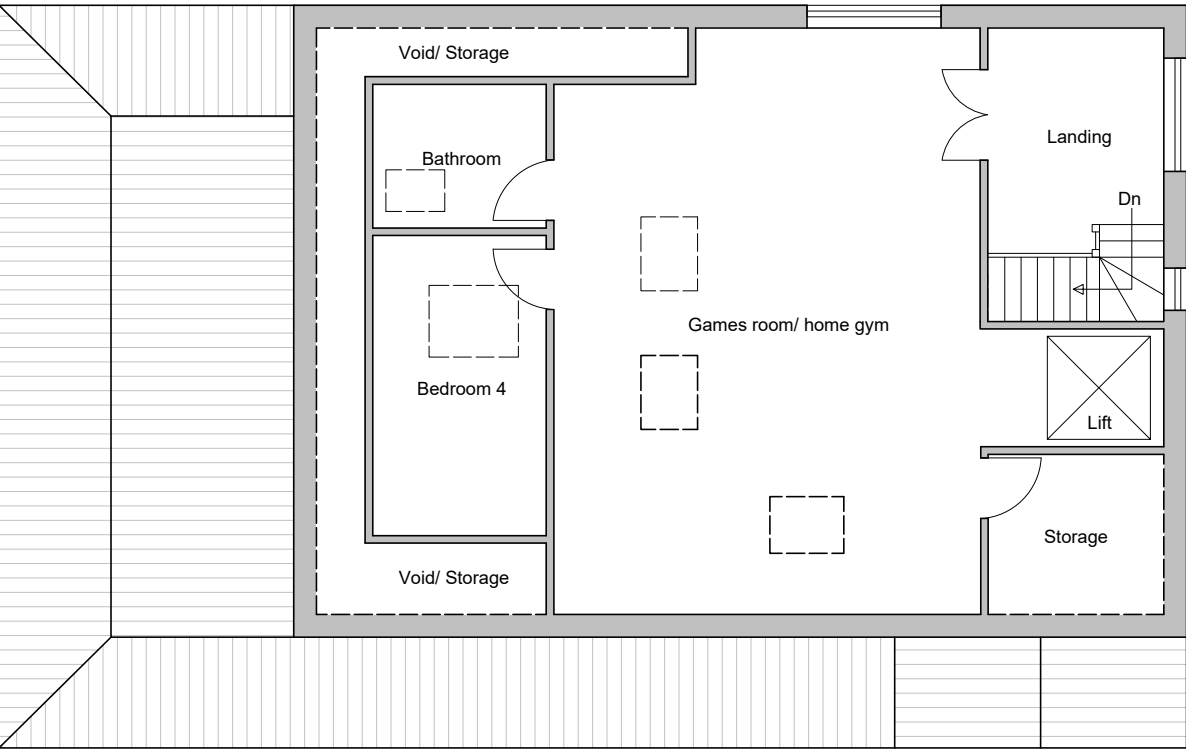
'As PROPOSED' SECOND FLOOR PLAN
