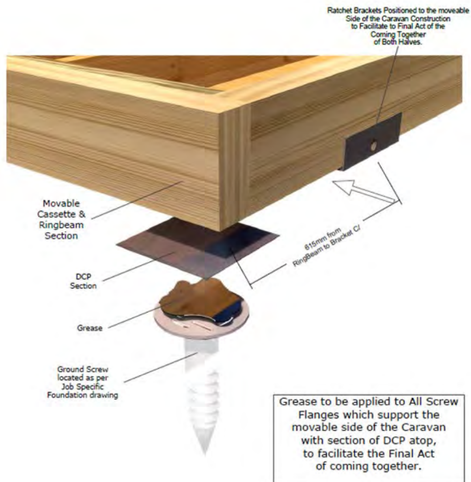
Ground Screw Illustration
