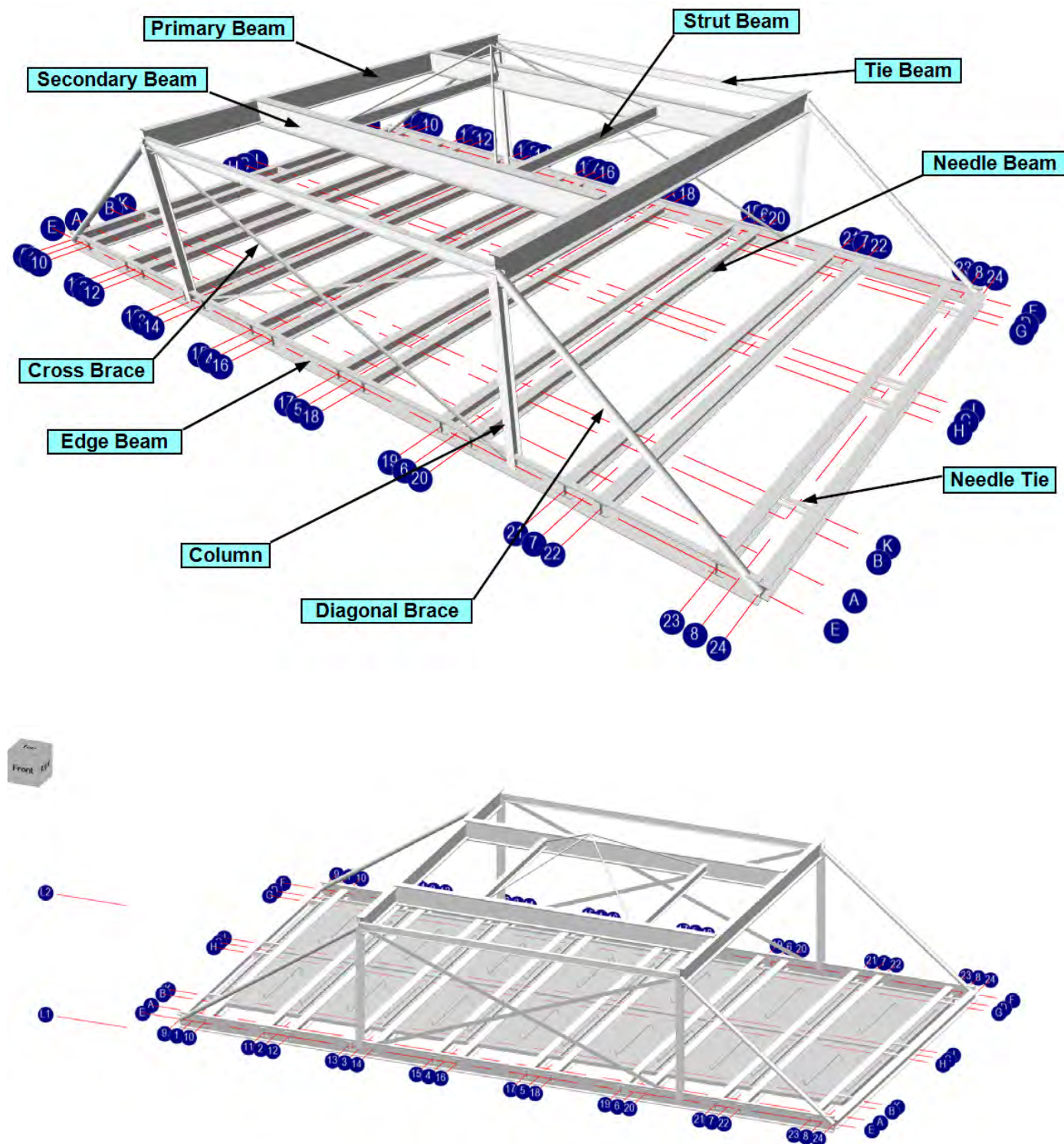
Lifting Frame for Flat Roofed Building
