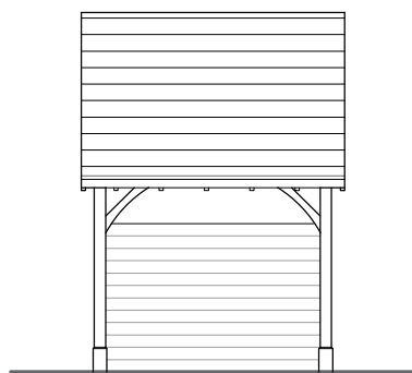
Elevation C
