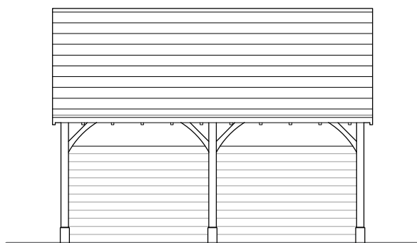
Elevation C
