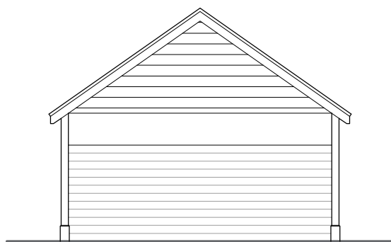
Elevation D
