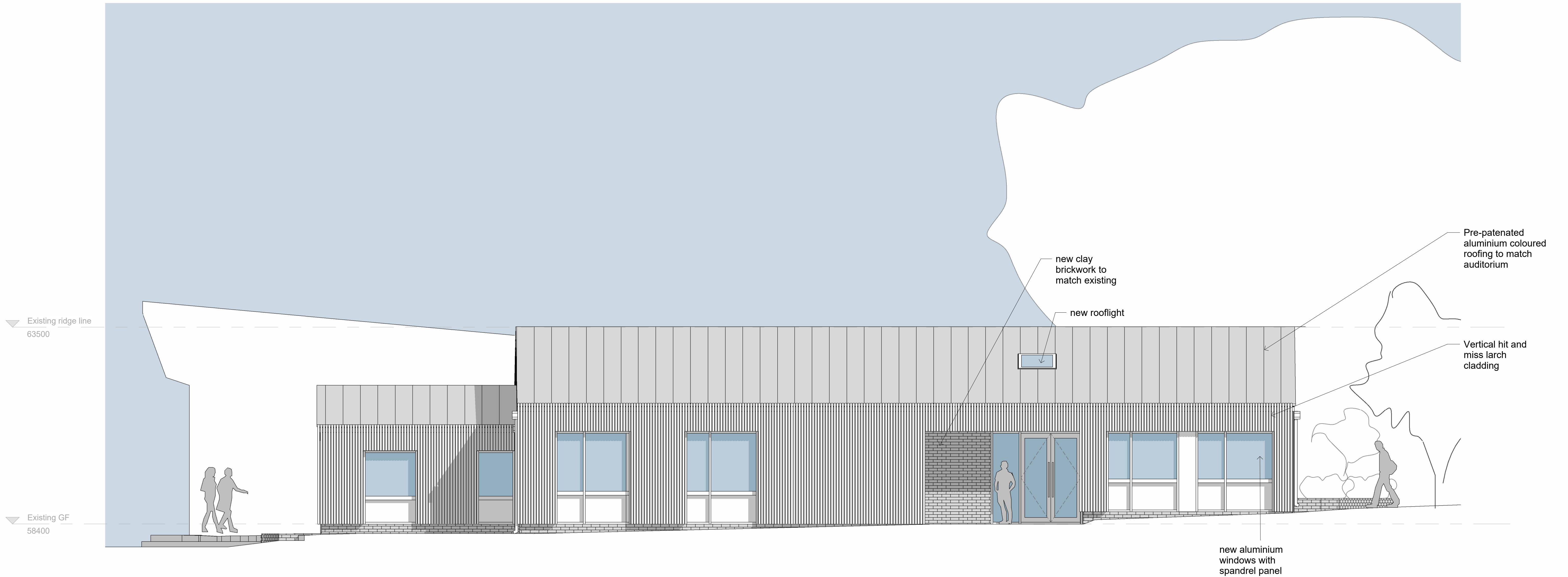
Proposed North (Way Hall side) 1 : 50
