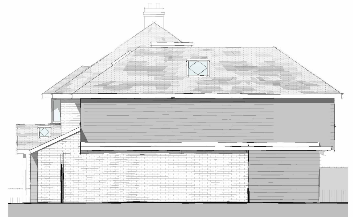
Side Elevation
