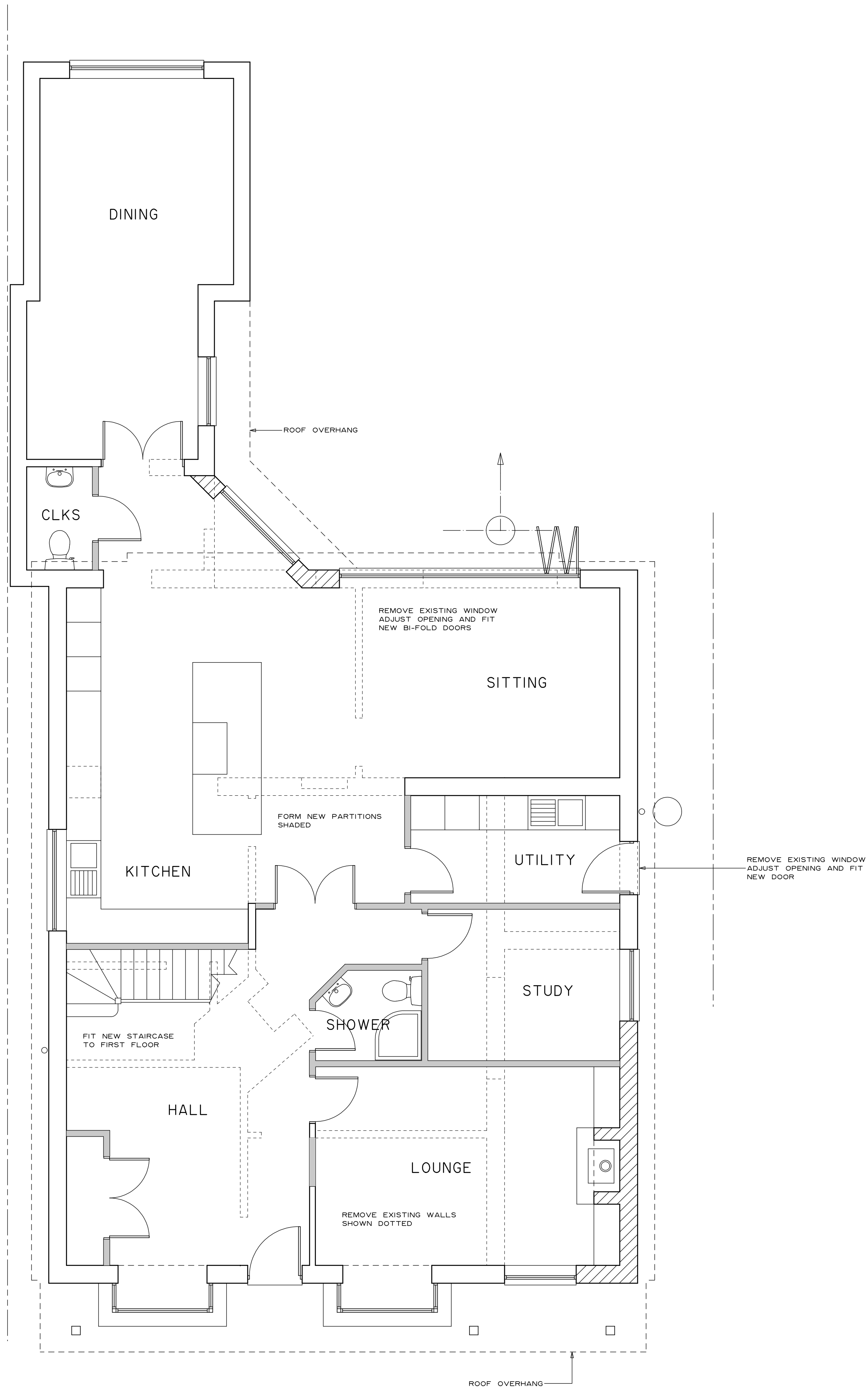
GROUND FLOOR
