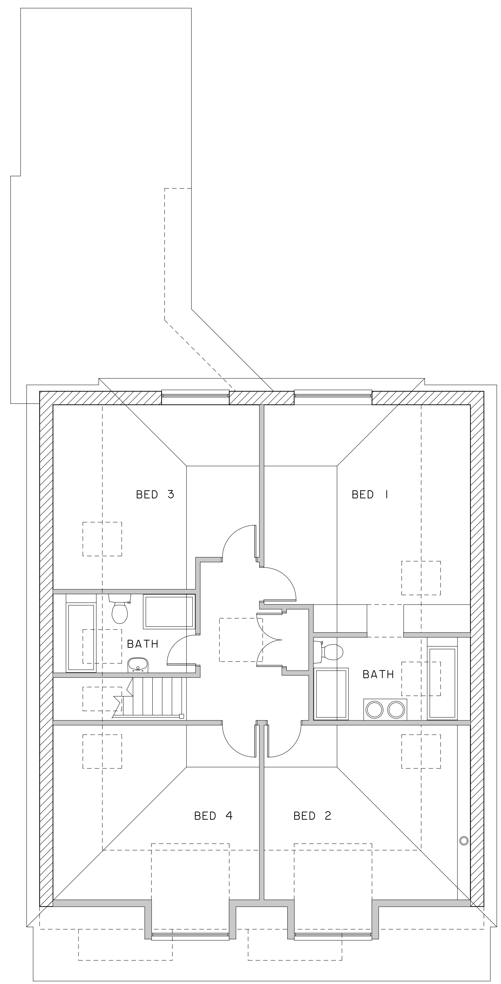
FIRST FLOOR
