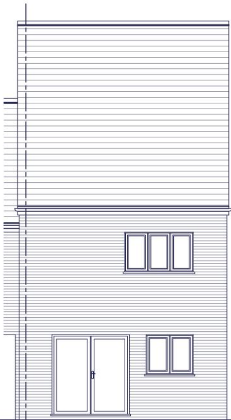
REAR ELEVATION
