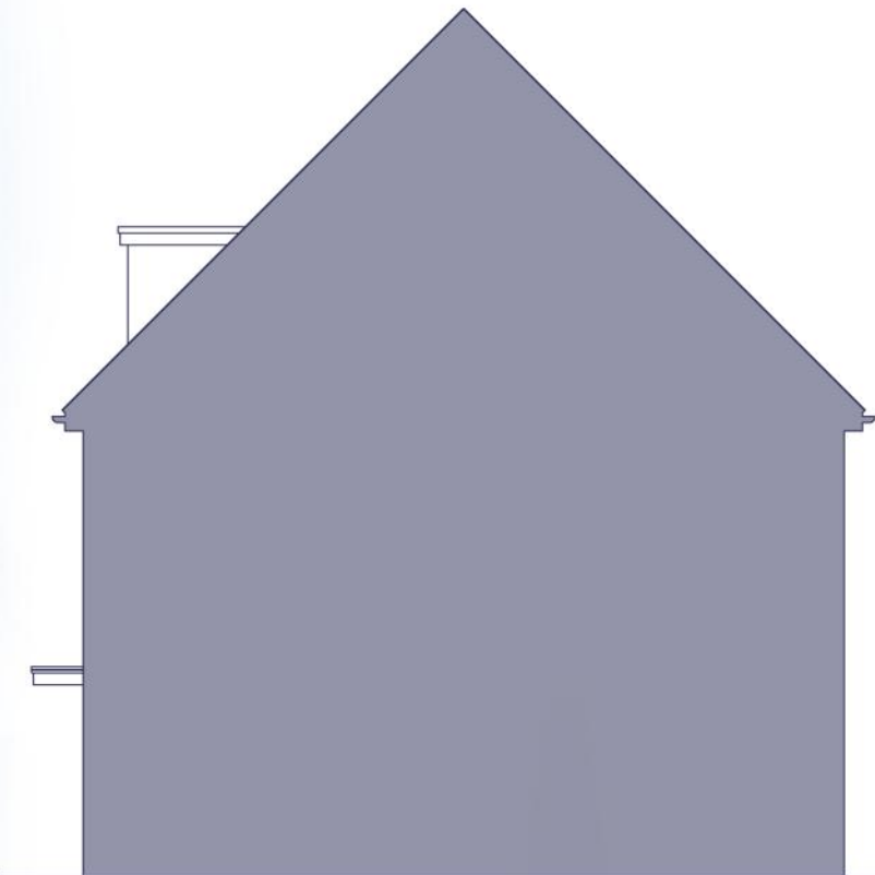
SIDE ELEVATION
