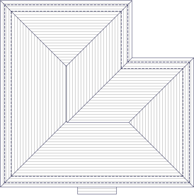
ROOF PLAN
