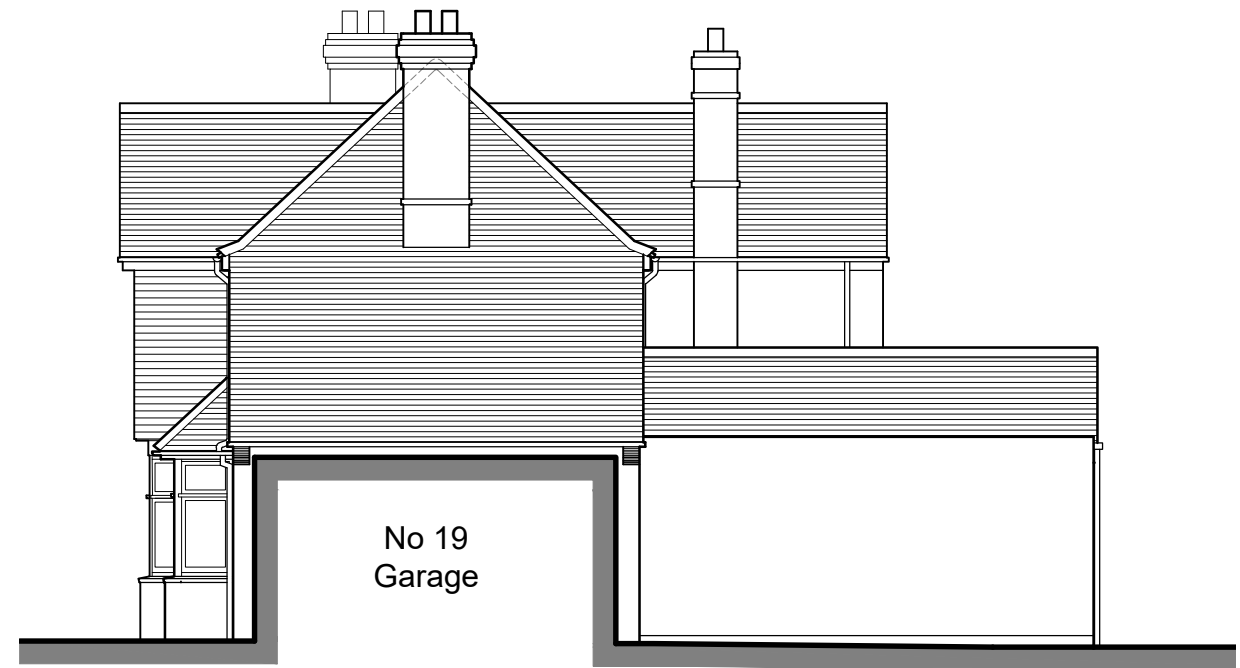
South Elevation
