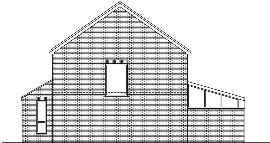
Existing Right Side Elevation Scale: 1/100
