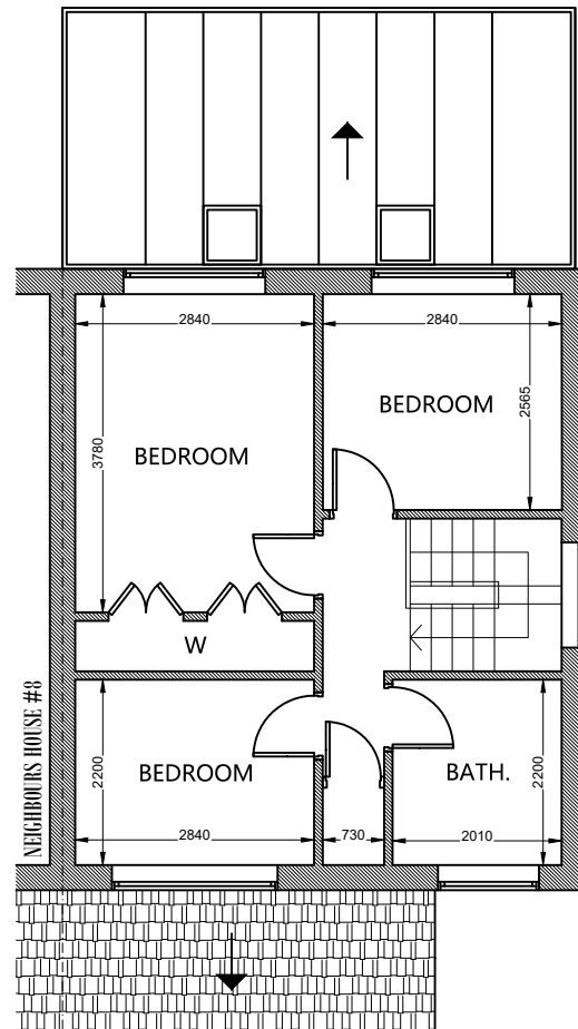
Pre-existing First Floor Plan Scale: 1/100
