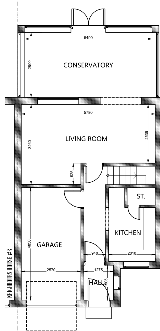
Pre-existing Ground Floor Plan Scale: 1/100
